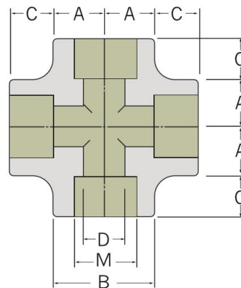
Cross
