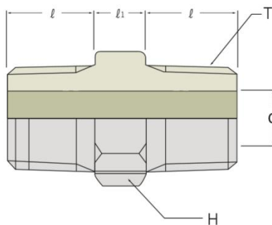
Hex. Nipple
