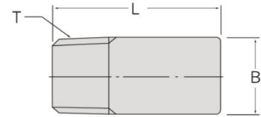
Round Plug
