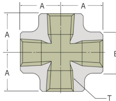
Cross
