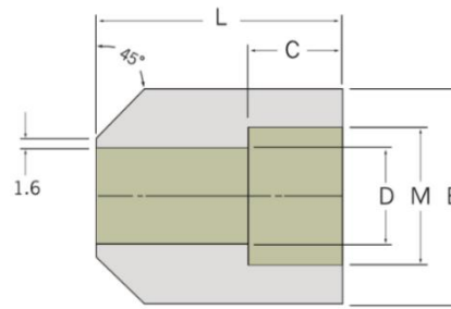
Boss
